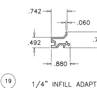
19 1/4" INFILL ADAPTER
