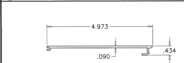
6 OPEN BACK FILLER
