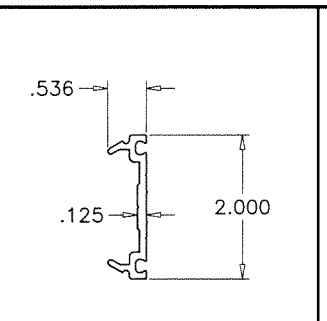
16 PRESSURE PLATE
