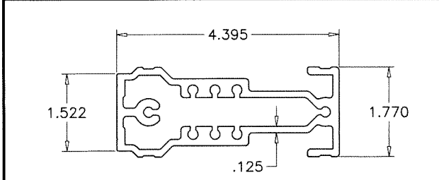
12 SHEAR BLOCK (INTERMEDIATE)
