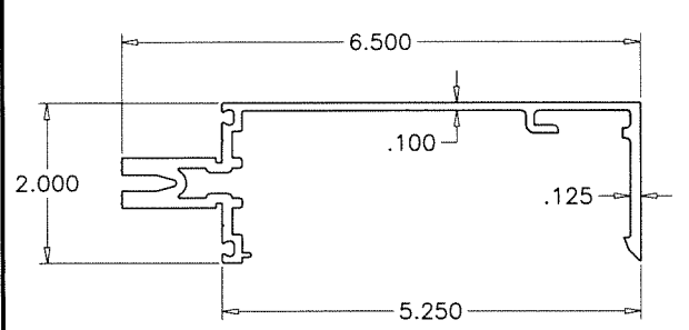
13 OPEN BACK HORIZONTAL
