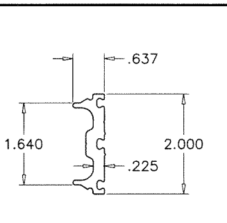
14 F/G PRESSURE PLATE
