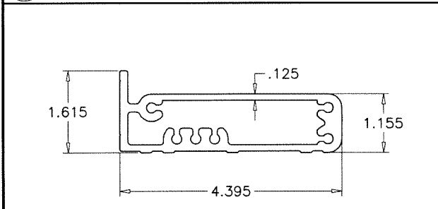
7 SHEAR BLOCK (HEAD/SILL)
