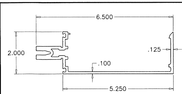
8 OPEN BACK HEAD/SILL
