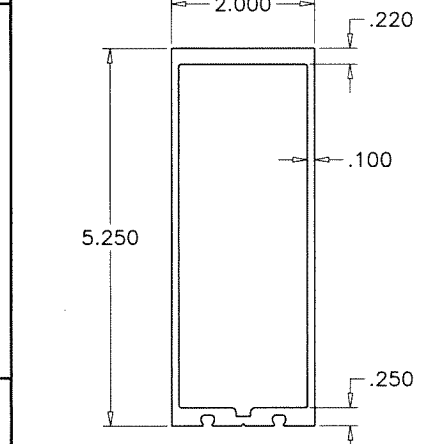
17 SSG HEAVY MULLION
