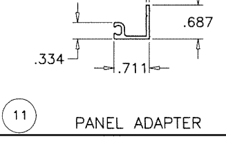
11 PANEL ADAPTER
