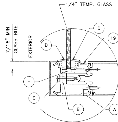
GLAZING DETAIL MONOLITHIC GLASS
